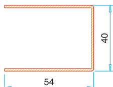
Door Sash 100 mm 3 Chambers Reinforcement
