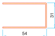
Door Sash 100 mm 4 Chambers Reinforcement
